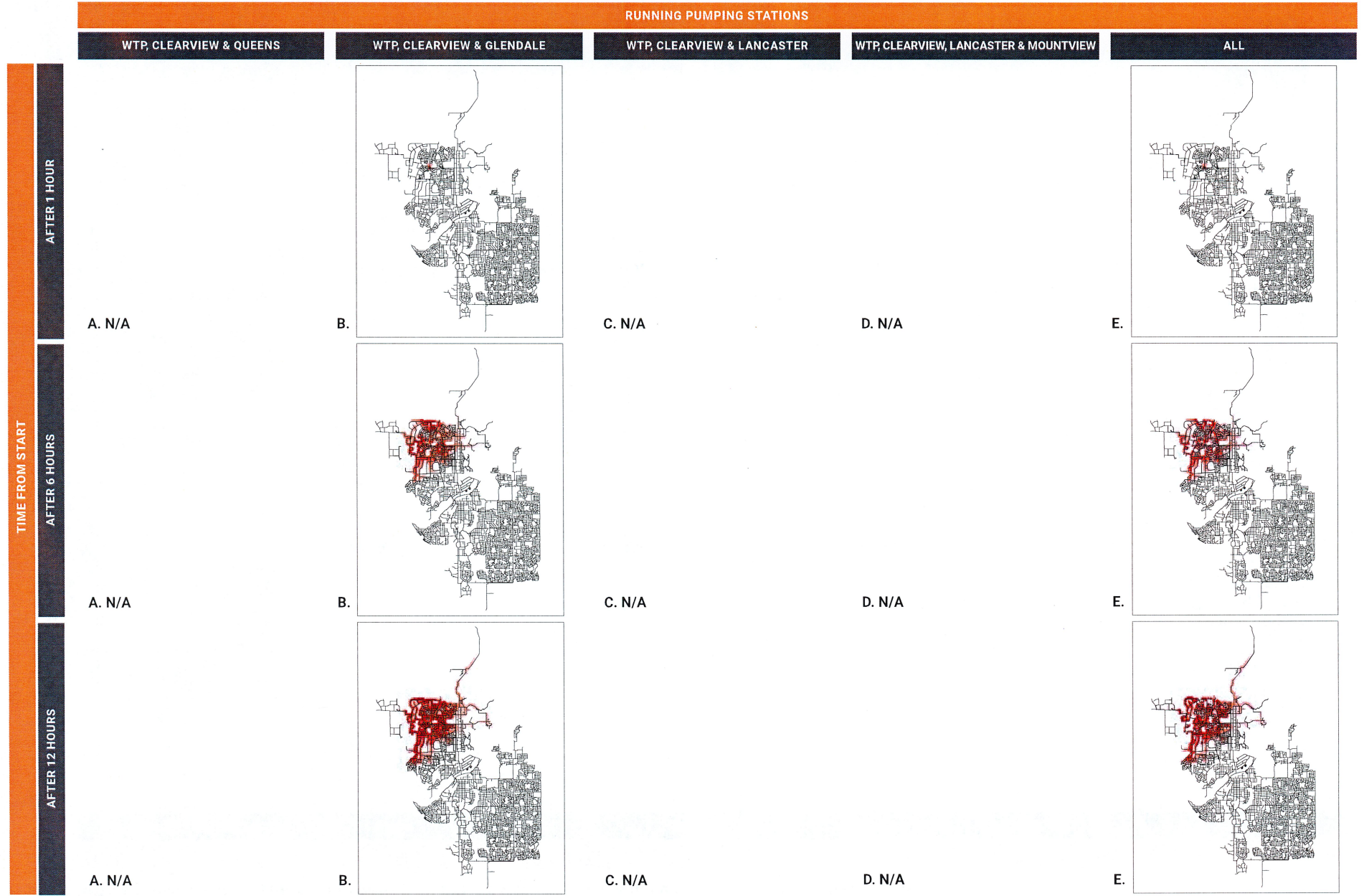
Figure C.4: Trace Analysis Results for the Glendale Pumping Station as the Trace Source under Average Day Demand Scenario
