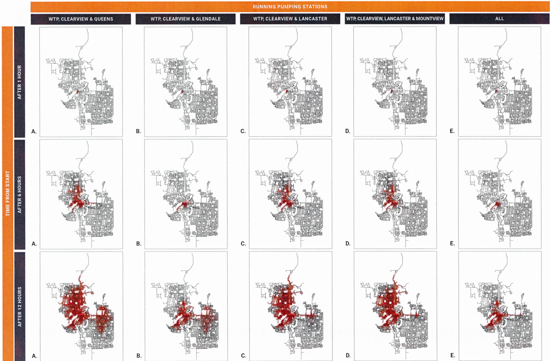
Figure C.1: Trace Analysis Results for the Water Treatment Plant as the Trace Source under Average Day Demand Scenario
