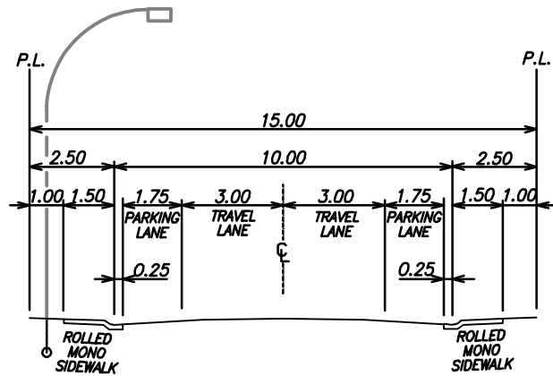
15/10 UNDIVIDED LOCAL ROADWAY
